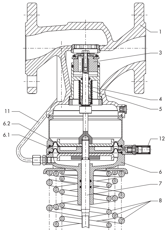
Type 44-3 Safety Shut-off Valve (SSV), flanged body version (DN 40)
