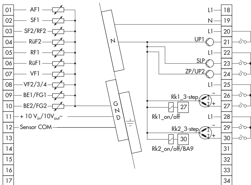
Fig. 3 · Terminal assignment of TROVIS 5573 Controller with standard back panel
